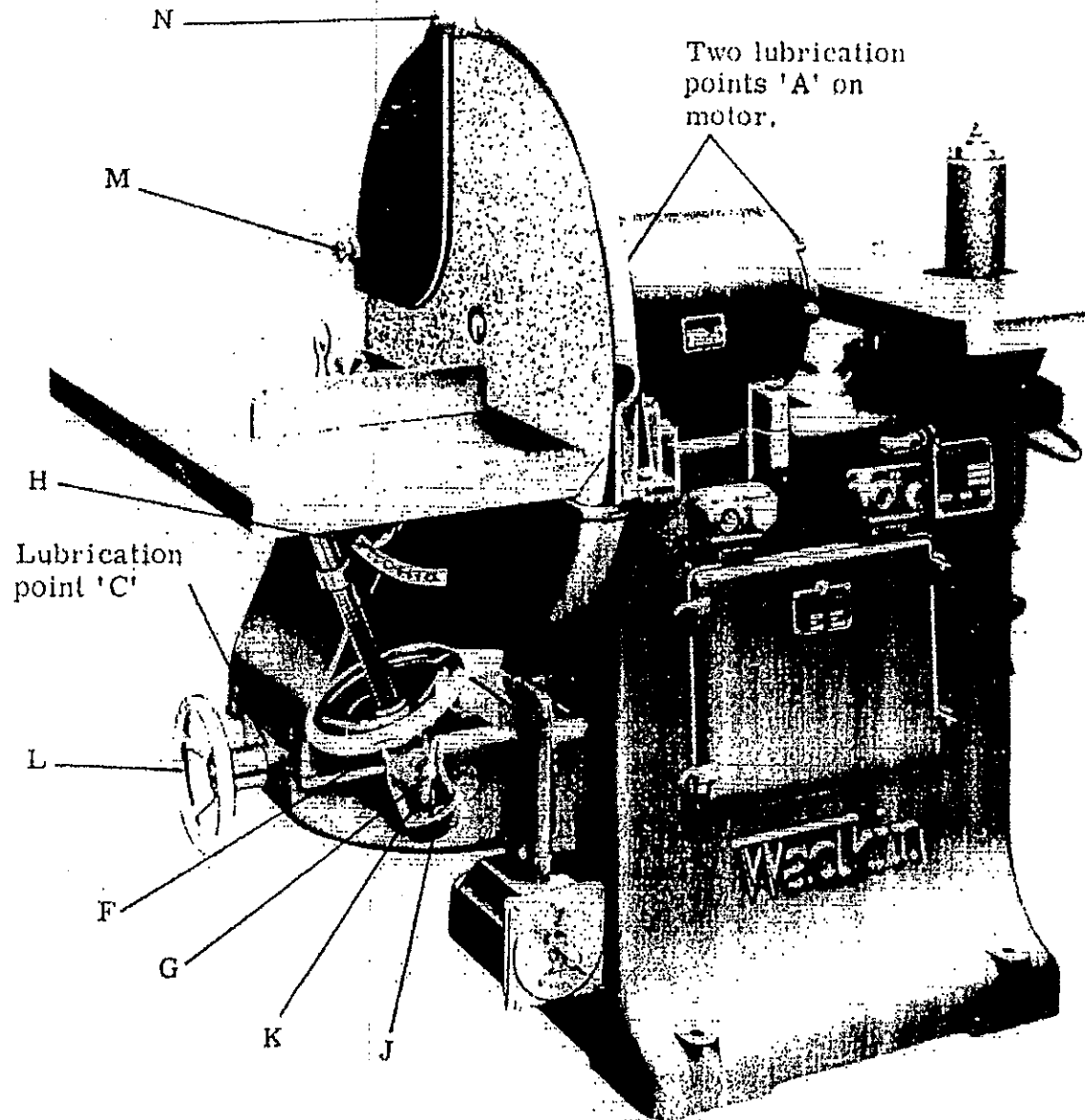
FIG. 1. FRONT VIEW OF MACHINE
